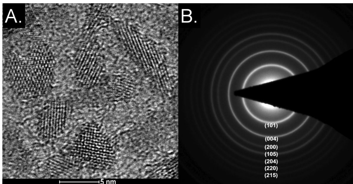
Figure 2. (A) TEM image of the TiO 2 NPs shows the presence of elongated crystalline particles. (B) Electron diffraction pattern obtained from the TiO 2 NP-s. The diffraction pattern indicates that the anatase particles are crystalline. 19
