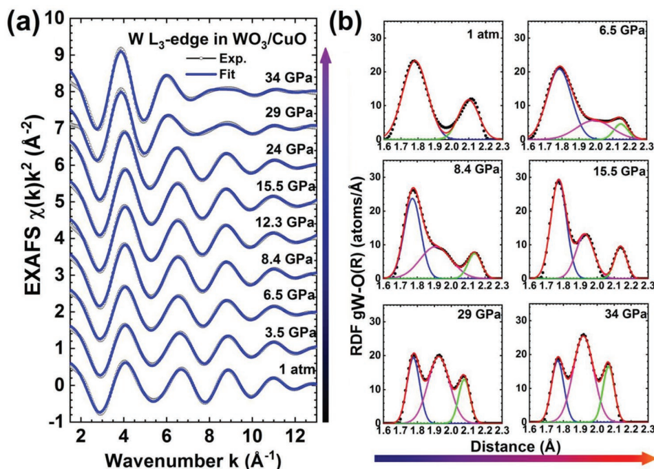
Figure 5. a) The pressure dependence of the experimental and calculated \text{W L}_3 -edge EXAFS for the first coordination shell of tungsten. b) Decomposition of the RDFs g_{\text{W-O}}(R) (solid circles) for the first coordination shell of tungsten into Gaussian components (solid lines). A variation of the \text{WO}_6 octahedra distortion upon compression is well observed.
