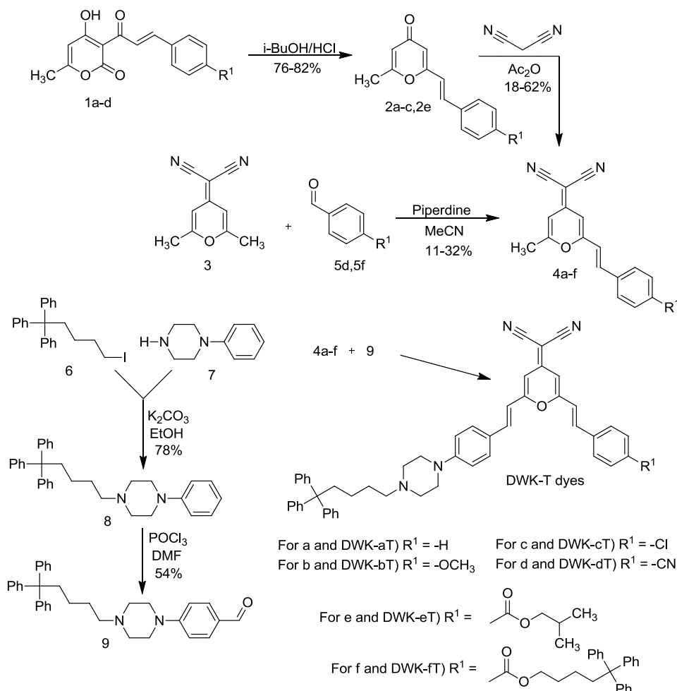
Fig. 1 Synthesis of nonsymmetric bis-styryl-DWK-type glassy dyes.
