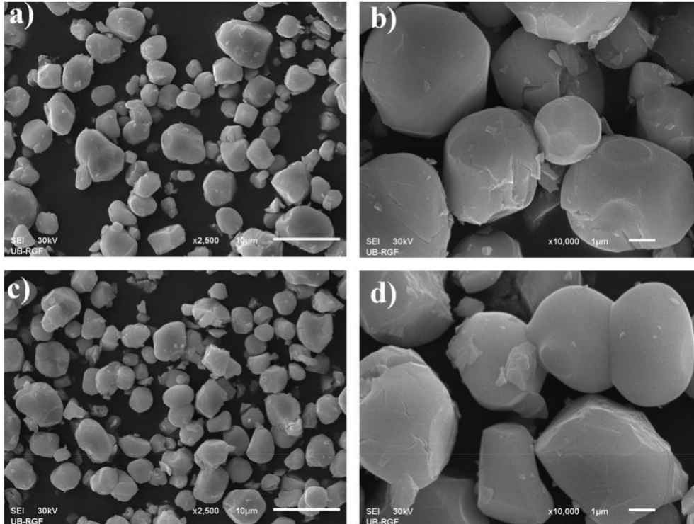
Fig. 2. SEM images of: (a, b) Er 3+ /Nd 3+ - and (c, d) Ho 3+ /Nd 3+ -doped GdVO 4 samples at different magnifications.
