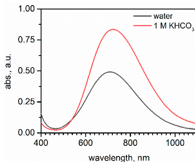
Figure 4. Electronic spectra of copper lactate complexes (16 mM) in water (pH = 8.5) and 1 M \text{KHCO}_3 solution (pH = 8.16).
