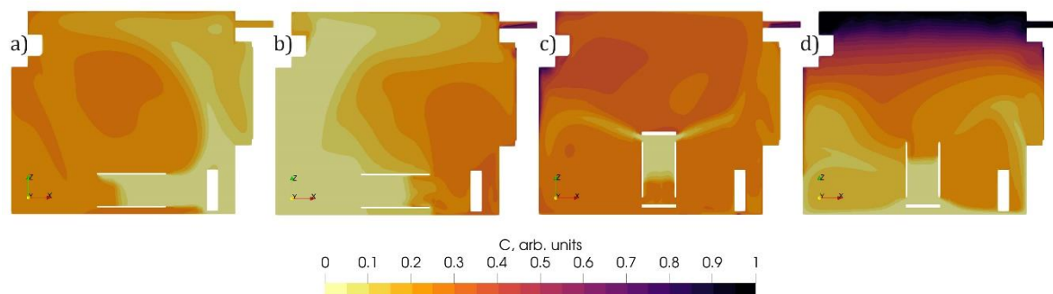
Fig. 1. Concentration distributions in the 3 \times 3 \times 3 \text{ m}^3 room after 400 seconds, starting with a uniform C_0 = 1 . Four different air cleaner cases with four different heating regimes are shown. Case a) the room is heated by an air-air heat pump / conditioner and purifier flow is in +x direction; case b) heated floor and purifier flow in -x direction; case c) radiator and upward purifier flow with top lid; case d) heated ceiling and downward purifier flow direction.
