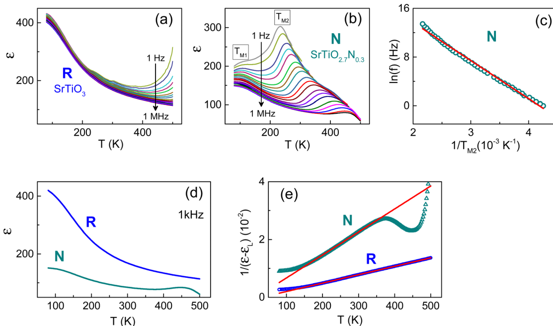
Fig. 2 Dielectric properties of the regular SrTiO 3 (R) and nitrogen-doped SrTiO 2.7 N 0.3 (N) polycrystalline STO films. (a), (b) and (d) The real part of the dielectric permittivity \epsilon as a function of temperature at different frequencies (a) and (b) f = 1\text{--}10^6 Hz and (d) f = 1 kHz. In (a) and (b), arrows show directions of frequency increase. (c) The frequency-temperature relationship for the dielectric peak at T_{M2} in the nitrogen-doped film. Straight line shows fit [ \ln(f) \propto 1/T_{M2} ]. (e) The modified Curie-Weiss behaviour ( f = 1 kHz). Straight solid lines show fits [ 1/(\epsilon - \epsilon_\infty) \propto T ].
