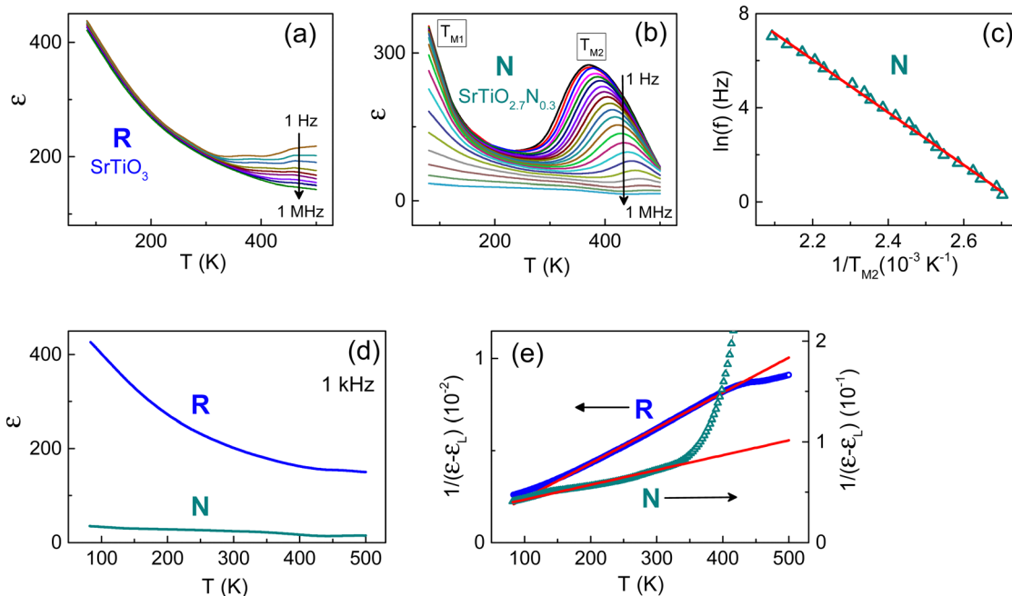
Fig. 3 Dielectric properties of the regular SrTiO 3 (R) and nitrogen-doped SrTiO 2.7 N 0.3 (N) homoepitaxial (001) STO films. (a), (b) and (d) The real part of the dielectric permittivity \epsilon as a function of temperature at different frequencies (a) and (b) f = 1\text{--}10^6 Hz and (d) f = 1 kHz. In (a) and (b), arrows show directions of frequency increase. (c) The frequency-temperature relationship for the dielectric peak at T_{M2} in the nitrogen-doped film. Straight line shows fit [ \ln(f) \propto 1/T_{M2} ]. (e) The modified Curie-Weiss behavior ( f = 1 kHz). Straight solid lines show fits [ 1/(\epsilon - \epsilon_L) \propto T ].
