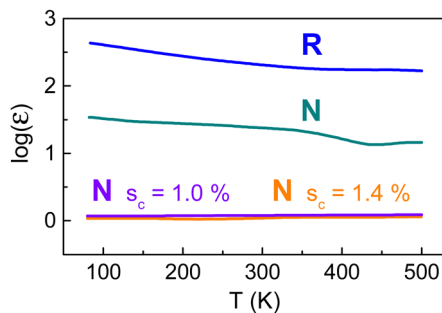
Fig. 4 Semi-log permittivity – temperature plots for the strained heteroepitaxial nitrogen-doped \text{SrTiO}_{2.7}\text{N}_{0.3} films (marked by “N s_c = 1.0\% ” and “N s_c = 1.4\% ”) compared to those for the homoepitaxial nitrogen-doped \text{SrTiO}_{2.7}\text{N}_{0.3} and regular \text{SrTiO}_3 films (marked by “N” and “R”, correspondingly). Frequency is 1 kHz.
