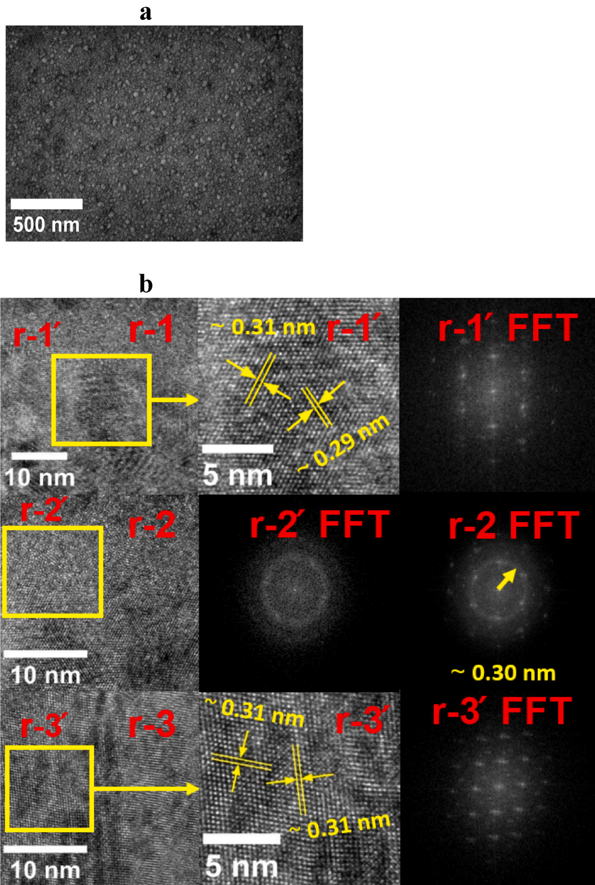
Fig. 4. a- HR-SEM image of S_6 . b- TEM images of S_6 ; Left column: r1, r2, and r3 are the different regions of the extracted lamella (separation \sim 50 nm). Middle column: r1', and r3' are the focused areas of the indicated regions in the left column and r-2' FFT is the fast Fourier transformation (FFT) of region r-2'. Right column: r-1' FFT, r-2' FFT and r-3' FFT are the fast Fourier transformations of the corresponding regions given in the left column.
