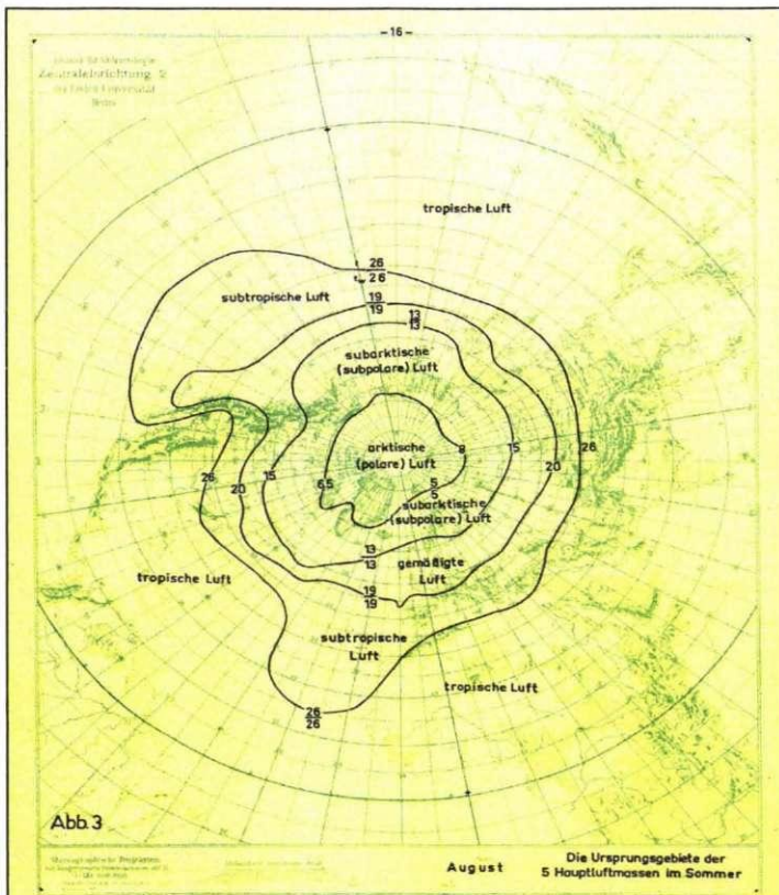
Figure 1-5. Areas of the origin of arctic, subpolar, temperate or mid-latitude (gemäßigte), subtropical and tropical air masses in the Northern hemisphere in winter (A) and summer (B). t/t_w – near surface air temperature/ temperature of water surface [after Geb, 1971]
