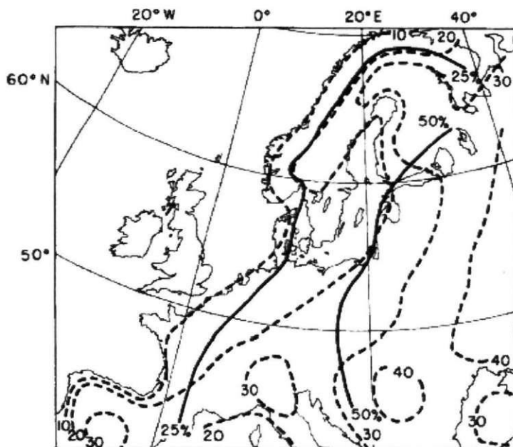
Fig. 5.1. Continentality in Europe. The indices of Gorczyński (dashed) and Berg (solid) are explained in the text (partly after Blüthgen 1966).
