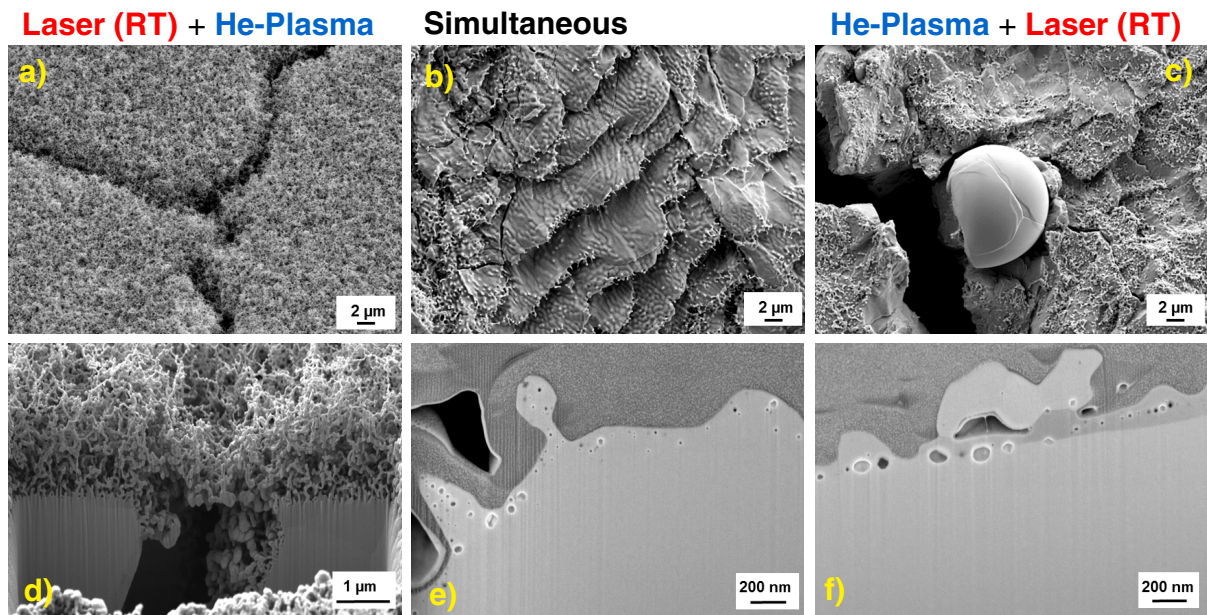
Figure 1. Scanning electron microscope images and focused ion beam cuts of He-plasma and laser-exposed surfaces: (a) and (d) First laser at room temperature, then He plasma exposure at 1120 K; (b) and (e) simultaneous laser and He-plasma exposure at 1120 K; (c) and (f) First He plasma at 1120 K then laser exposure at room temperature [20]. Reproduced from [20]. CC BY-NC-ND 4.0.
