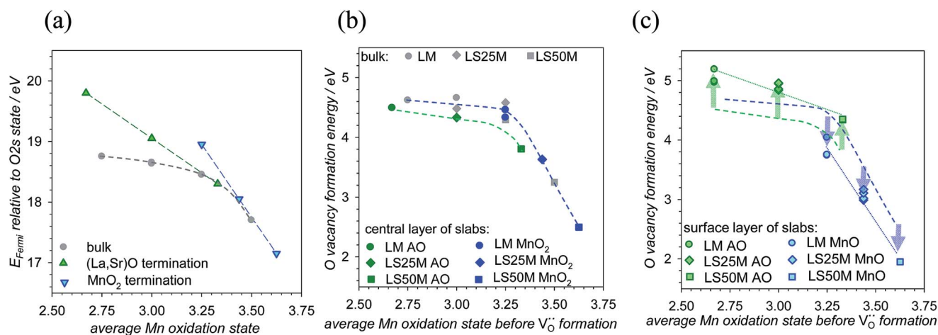
Fig. 3 (a) The Fermi level energy relative to the O 2s deep states for bulk and 7-layer slabs, and the different formal average Mn oxidation states are caused by different V O •• concentrations (bulk) as well as La/Sr ratios (bulks and slabs). (b) Oxygen vacancy formation energy E_{V_O} in the bulk and in the central layer of (001) (La,Sr)O and (001) MnO 2 terminated 7-layer slabs. (c) E_{V_O} in the surface layers of (001) (La,Sr)O and (001) MnO 2 terminated 7-layer slabs, and the dashed lines indicate E_{V_O} of the respective central layers from (b).
