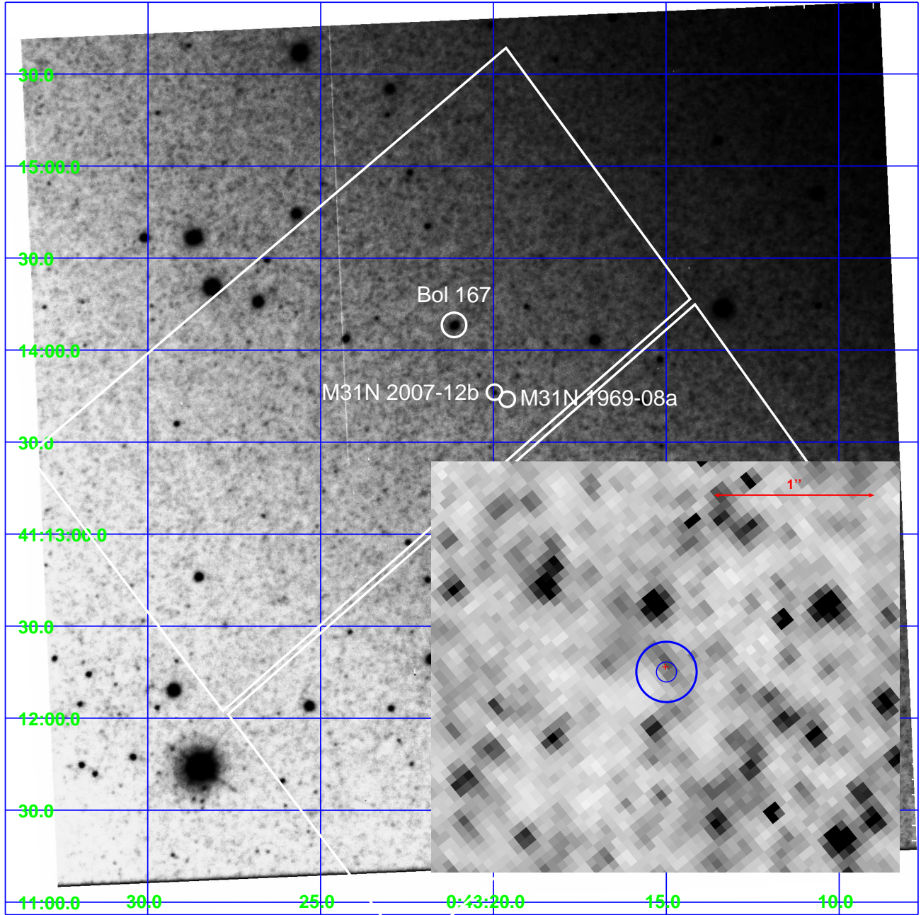
FIG. 3.— Main image: Liverpool Telescope Sloan- i' image of M31N 2007-12b taken on 2007 December 14.95 UT, field 4.6' \times 4.6' . The position of M31N 2007-12b and the new position of M31N 1969-08a are shown by the small white circles (left and right respectively, circles have a diameter of 5'' ). The white boxes indicate the approximate positions of the HST ACS-WFC field. Also shown is the position of the nearby globular cluster Bol 167. Inset: HST ACS-WFC image of the \sim 3' \times 3' region surrounding M31N 2007-12b. The inner blue circle indicates the 1\sigma ( 1.25'' ) radius search region for the progenitor, the outer circle the 3\sigma region, the red cross indicates the position of the progenitor candidate.
