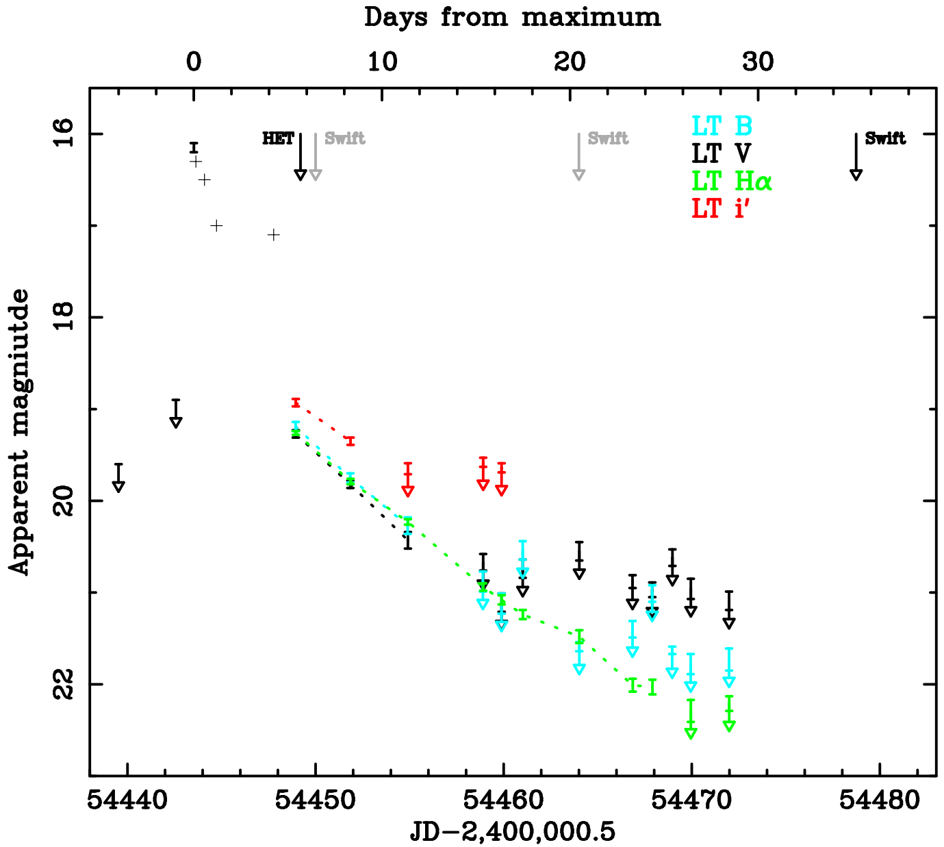
FIG. 1.— The optical light curve of M31N 2007-12b with data from Lee et al. (2007) and the “M31 (Apparent) Nova Page” provided by the International Astronomical Union, Central Bureau for Astronomical Telegrams (CBAT - http://www.cfa.harvard.edu/iau/CBAT_M31.html ) comprising both R band and unfiltered CCD observations, plus data from the Liverpool Telescope (data points from t \sim 5 days after peak and in photometric bands as indicated). Times of Swift observations (upper limits grey; detection at t = 35 days bold) and HET spectroscopy are also shown.
