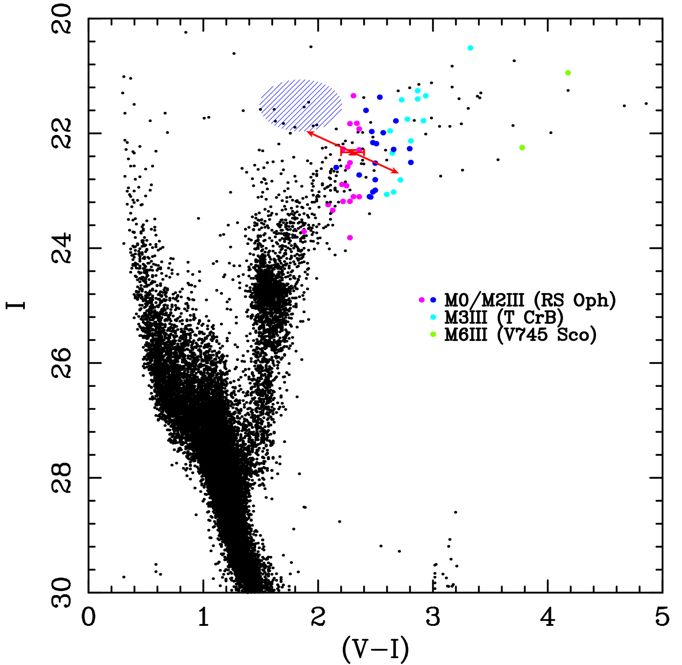
FIG. 4.— Color-magnitude diagram showing the Hipparcos data-set (Perryman & ESA 1997), with parallax and photometric errors < 10\% . The Hipparcos stars have been moved to the position of M31 assuming (m - M)_0 = 24.43 (Freedman & Madore 1990) an estimated extinction towards M31 of E_{B-V} = 0.1 mag (Stark et al. 1992) and an internal extinction of E_{B-V} = 0.25 . The red point shows the candidate for the progenitor of M31N 2007-12b. The colored points are known M0/M2III (RS Oph), M3III (T CrB) and M6III (V745 Sco) secondary stars of RNe (Anupama 2008). The dark blue hatched ellipse shows the location of a quiescent RS Oph system (with the major and minor axes of the ellipse relating to 1\sigma scatter from the mean). The red arrow shows the extent of the likely effects of internal extinction ( \Delta E_{B-V} = \pm 0.25 ).
