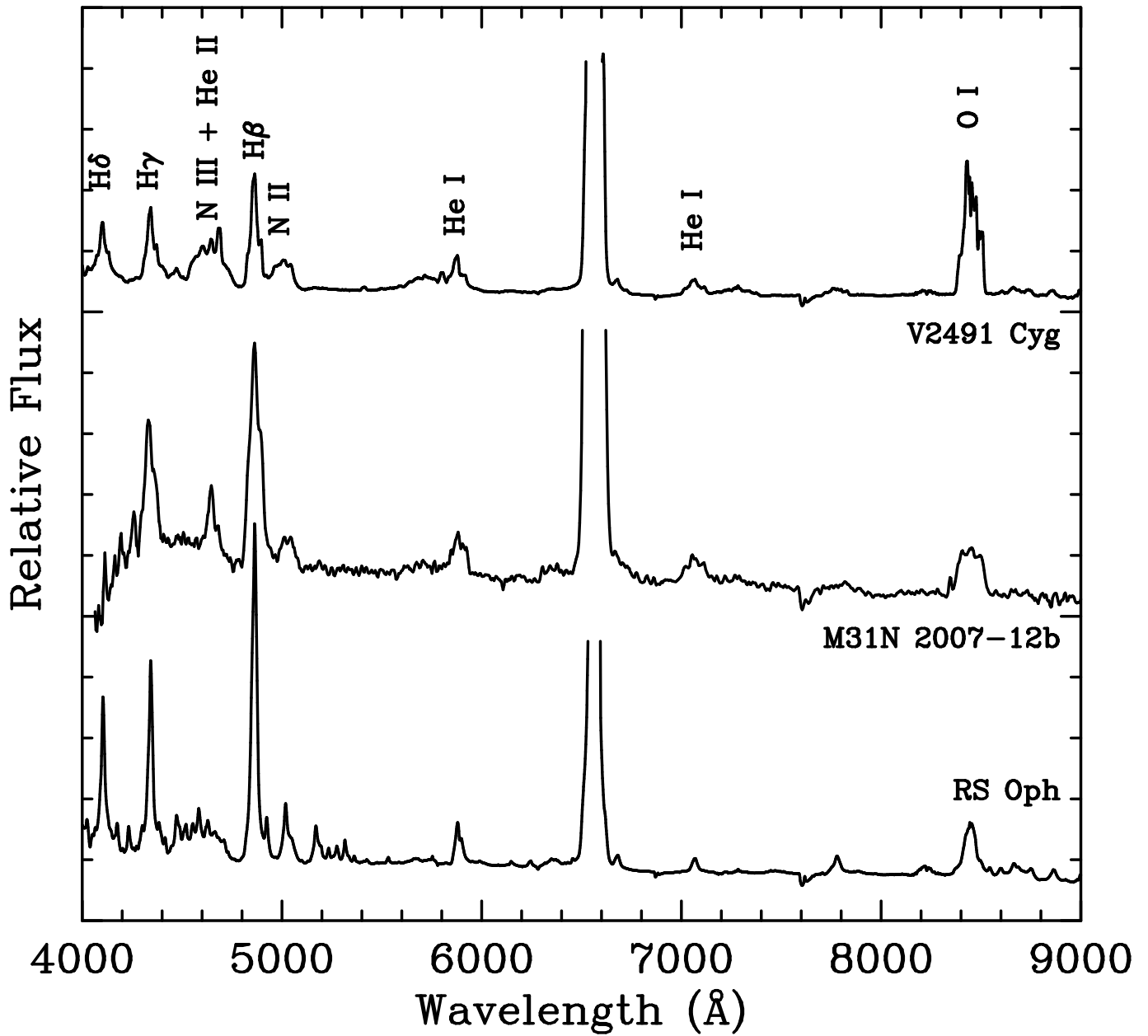
FIG. 2.— Low resolution spectrum of M31N 2007-12b taken with the LRS on the HET at t = 5.2 days after discovery. The spectrum would classify this object as a He/N Classical Nova following maximum light. Also shown for comparison are spectra of the Recurrent Nova RS Oph at around 6 days from outburst (Anupama 2008) and the supposed RN V2491 Cyg (from two co-added spectra at around 17 and 18 days after outburst, Anupama et al. in preparation) - see text for further details. The H \alpha line in each spectrum has been truncated.
