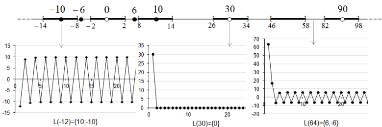
Figure 4. Illustration if x_0 \in \{-12; 30; 64\} .
