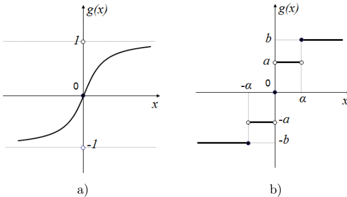
Figure 1. Simple step functions: a) sigmoid function g(x) = \frac{2}{\pi} \arctan x , b) step signal function g(x) .
