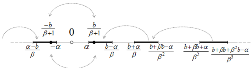
Figure 2. Illustration of Statement 1) of Theorem 4. Presentation of set \Omega_b .
