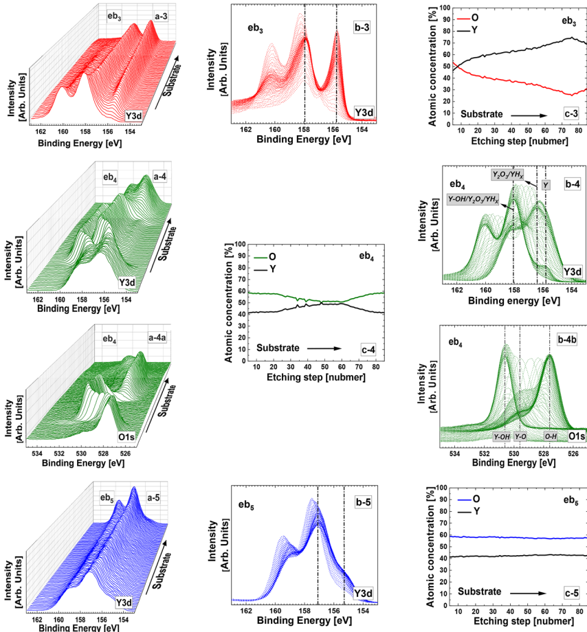
Figure 3: XPS depth profile of samples: eb_3 (metallic): (a-3)-depth-resolved Y3d spectrum dynamic in 3D, (b-3)-corresponding Y3d binding energy representation/density mapping of the spectrum in Figure 3a-3 in 2D, (c-3)-atomic concentration of yttrium and oxygen depending on depth. eb_4 (oxidized hydride): (a-4)-depth-resolved Y3d spectrum dynamic in 3D, (b-4)-corresponding Y3d binding energy representation/density mapping of the spectrum in Figure 3a-4 in 2D, (c-4)-atomic concentration of yttrium and oxygen depending on depth; (a-4a)-depth-resolved O1s spectrum dynamic in 3D, (b-4b)-corresponding O1s binding energy representation/density mapping of the spectrum in Figure 3a-4a in 2D, eb_5 (oxide): (a-5)-depth-resolved Y3d spectrum dynamic in 3D, (b-5)-corresponding Y3d binding energy representation/density mapping of the spectrum in Figure 3a-5 in 2D, (c-5)-atomic concentration of yttrium and oxygen depending on depth.
