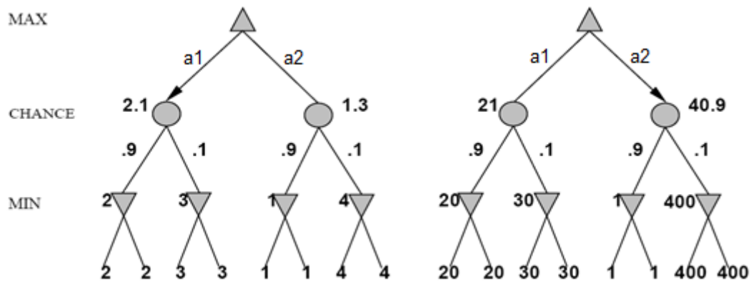
Figure 8. Positive linear transformation of evaluation function [11]
