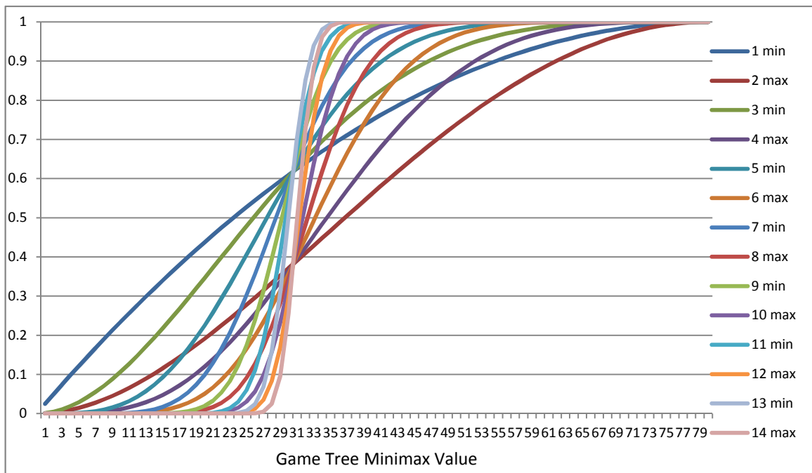
Figure 31. Cumulative probability function by level for depth 14
