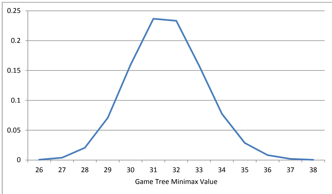
Figure 34. Resulting zoomed-in function
