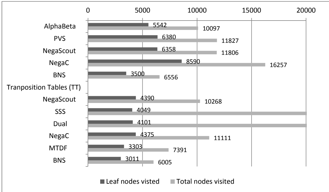
Figure 50. Tree width – 3, depth – 10
