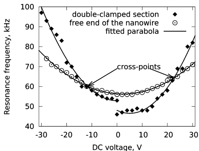
Fig. 5 Dependence of the resonant frequency of a Ge nanowire on the DC field applied between electrodes.
