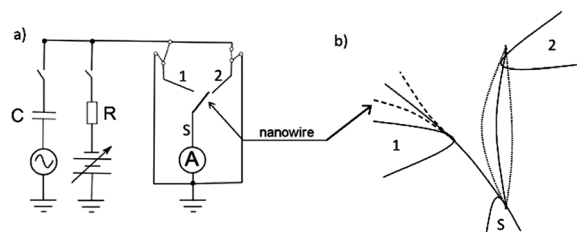
Fig. 2 (a) Schematic of the experiment set-up for reduced DC switching. The DC and AC fields can be applied between the selected source electrode and the nanowire tip separately or together. (b) Modes of the nanowire oscillation between electrodes 1, 2 and S.
