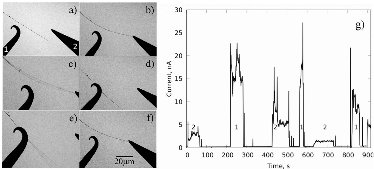
Fig. 4 Operation of a DC-AC field controlled nanowire switch. The operational DC field was 20 V: (a) the initial position of the nanowire between the source electrodes; (b) the nanowire in contact with electrode 2; (c) the double-clamped nanowire is resonating under the influence of an AC field. The AC amplitude is 2.75 V; (d) the nanowire switches to electrode 1 at an AC amplitude of 12.5 V; (e) the free end of the nanowire is resonating under the influence of an AC field. The AC amplitude is 1 V; (f) the nanowire switches to electrode 2 at an AC amplitude of 10 V; (g) the current-time characteristics of the device. Current jumps are labeled with numbers of the source electrode with which contact occurred.
