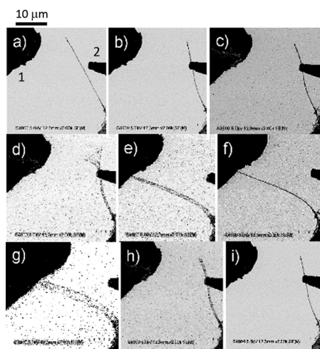
Fig. 3 (a–i) SEM images of the step-by-step operation of a two-source nanowire switch controlled by combined DC-AC fields.
