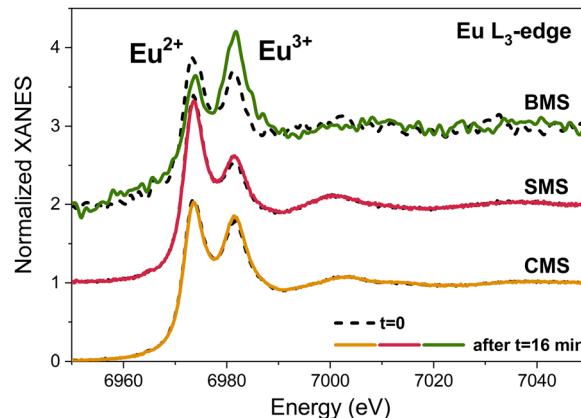
Fig. 2 The \text{Eu L}_3 -edge XANES spectra of polycrystalline CMS, SMS and BMS doped with 0.1% Eu. Dashed lines – spectra measured immediately after opening the beam shutter, solid lines – spectra collected after 16 minutes.
